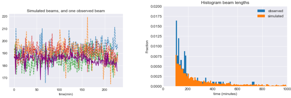
(a) Four simulated beams using Equation (6) and one observed beam in purple, all with same initial value I_0 .
