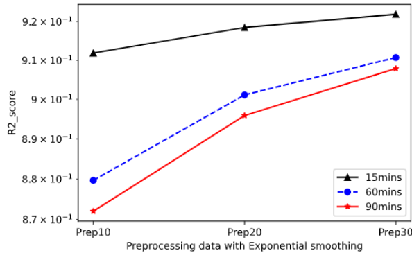
Figure 14: Using data preprocessed by three different windows to predict 15, 60 and 90 minutes ahead of “ITL.BCT05:CURRENT” target.
