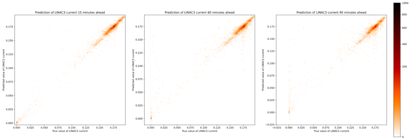
Figure 15: Results for the XGBoost for 15, 60 and 90 minute forecast with the 6 column set; Left ( R^2 : 0.9845, RMSE: 0.004988); Middle ( R^2 : 0.9588, RMSE: 0.007976); Right ( R^2 : 0.9458, RMSE: 0.009329)
