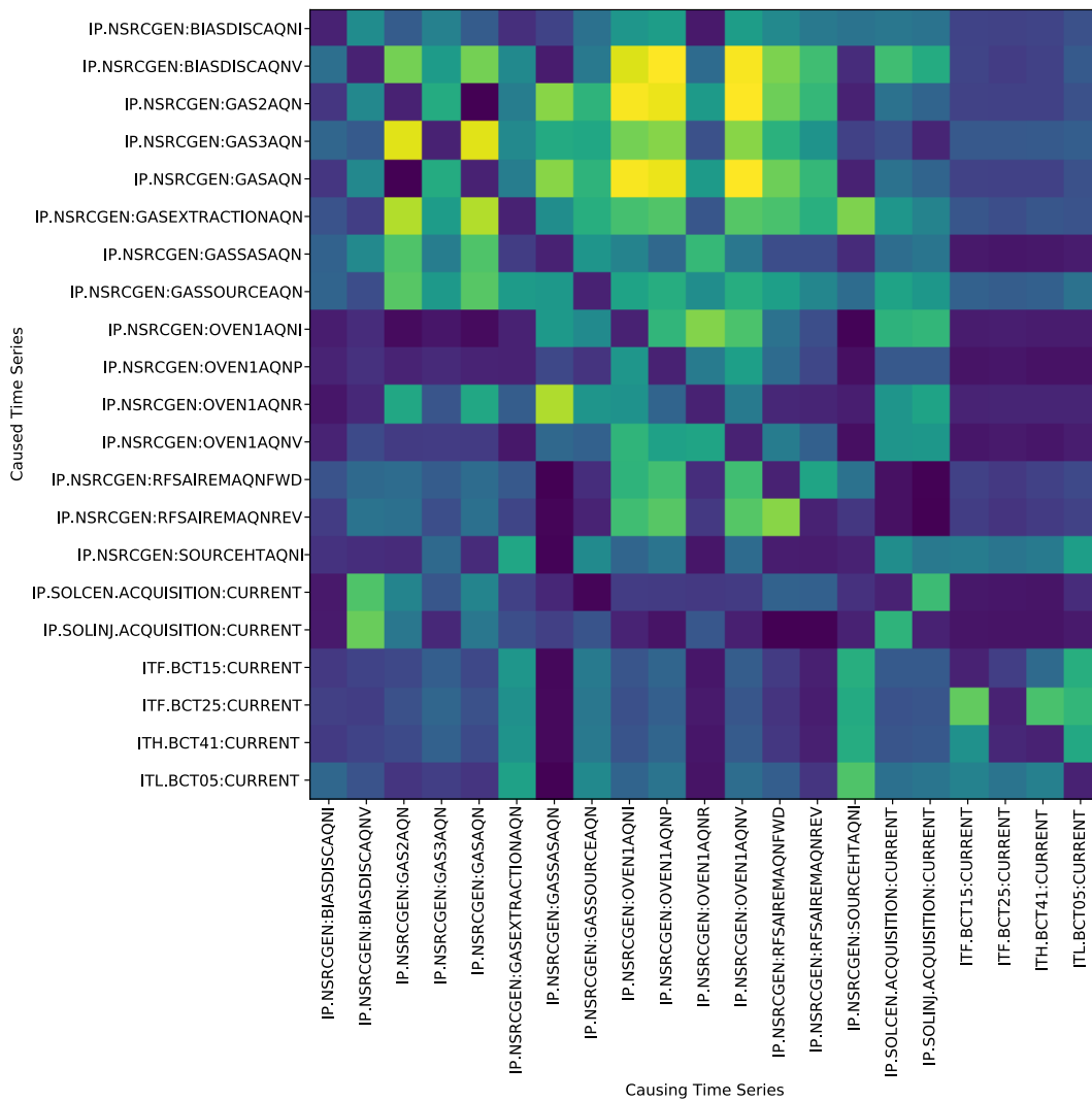
Figure 9: Log of Pairwise Granger Causality f -vals for all Columns, where lighter hues represent higher causality
