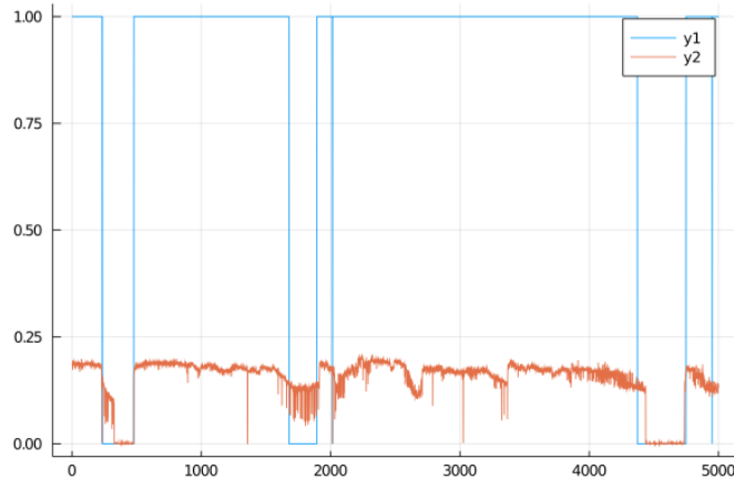
Figure 4: Ising Model Classification of Good/Bad Beams
