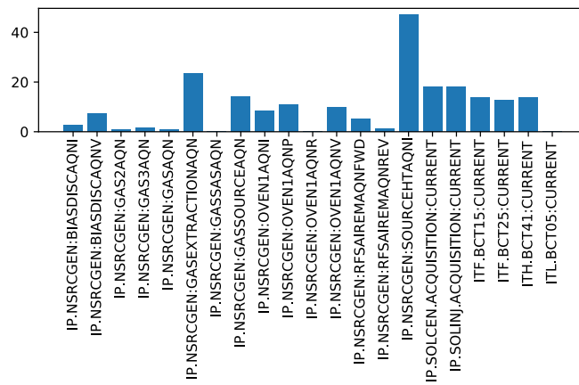
Figure 8: Granger Causality f -vals for Subset of Columns
