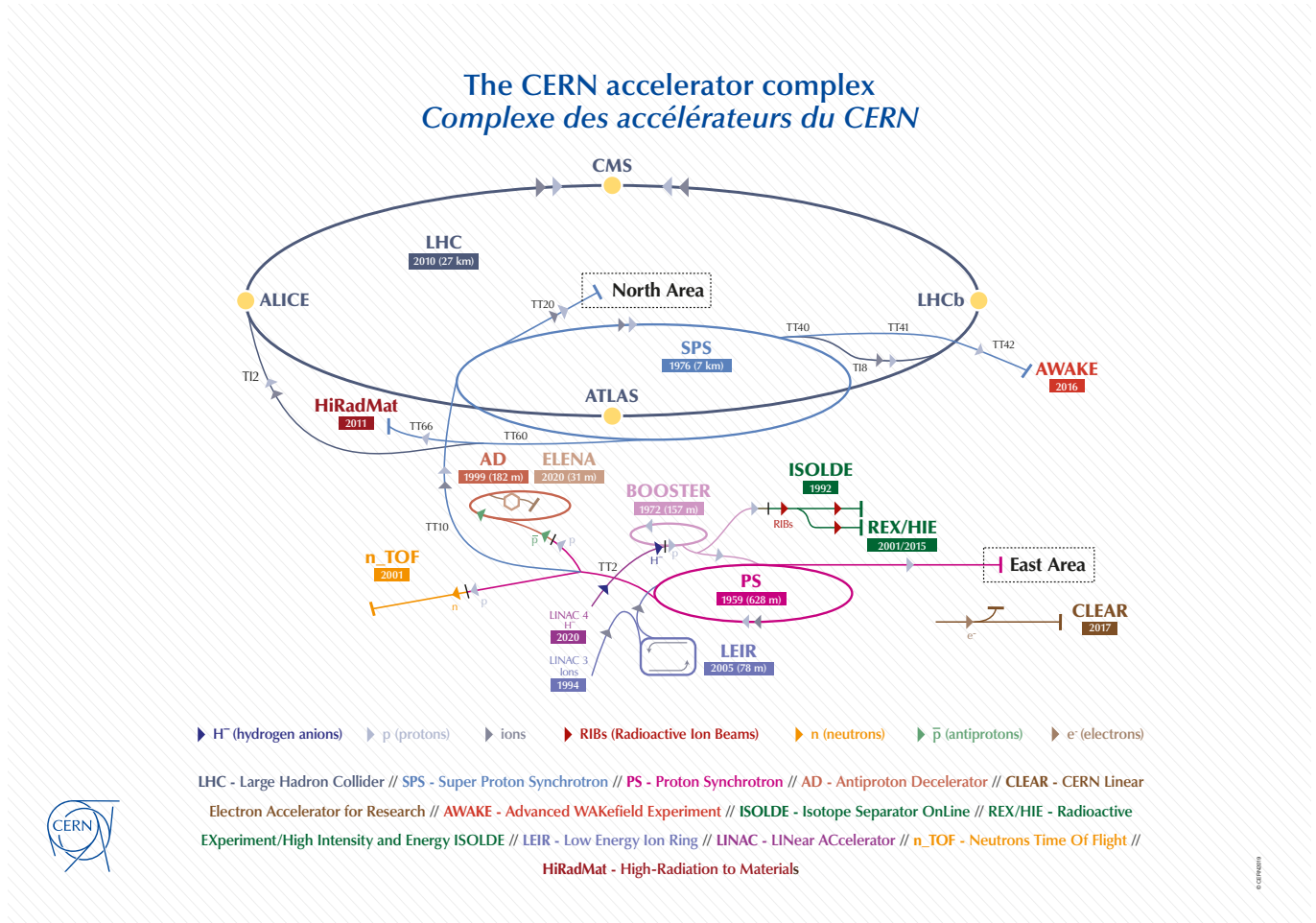
Figure 1: A schematic Of The Accelerator Complex
